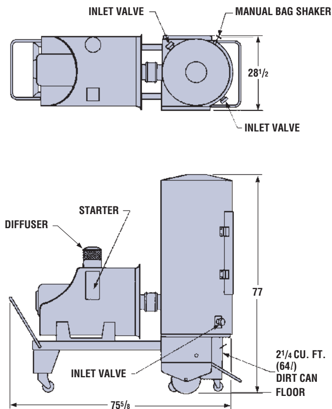
Mobile Model
