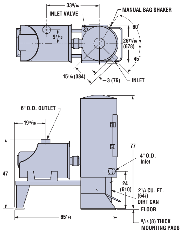
Stationary Model
